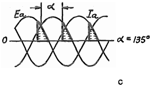
Fig. 45—Voltage conditions in 3-phase half-wave rectifier, with resistive load.
