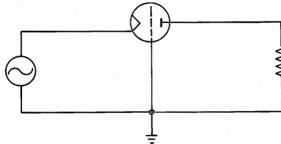
Fig. 5—Grounded-grid amplifier circuit.
