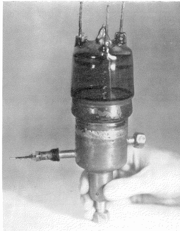
Fig. 8—25-watt tube, \lambda=5 centimeters.
