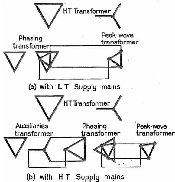
Fig. 52—Three-phase full-wave series rectifier circuit.
