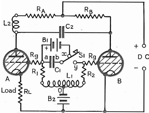
Fig. 24—Generator of square-wave single pulses.
