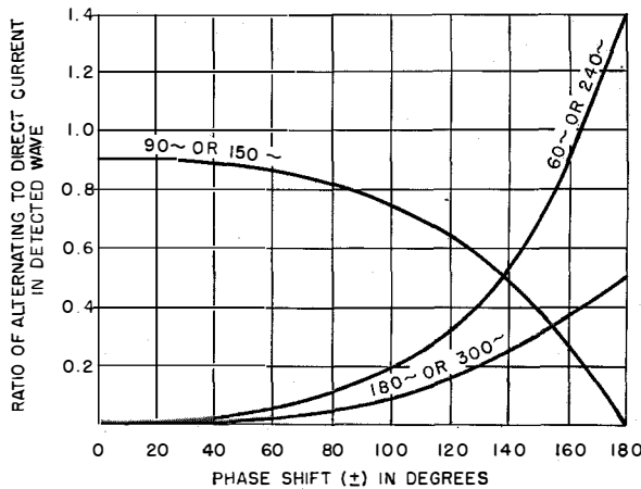
Fig. 45—Distortion in a modulated wave as a result of phase shift of carrier with respect to side bands.
