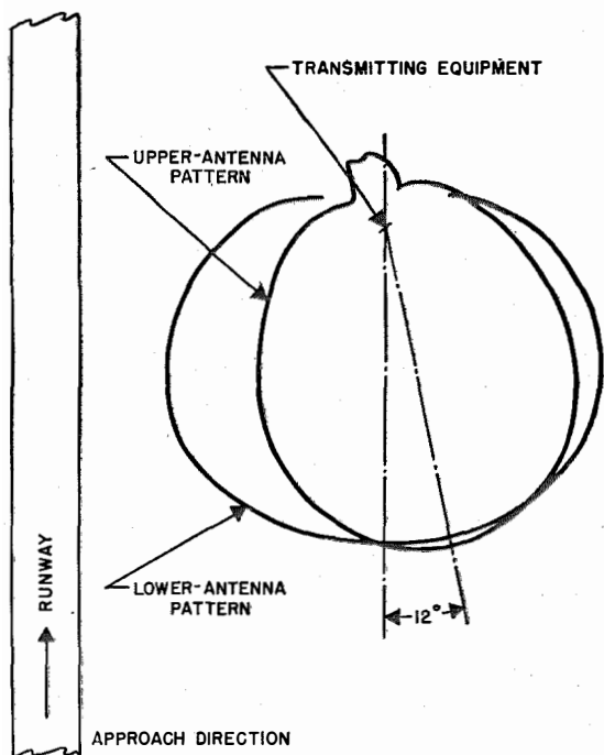
Fig. 24—Horizontal radiation patterns of upper and lower antennas measured at any glide-path angle.
