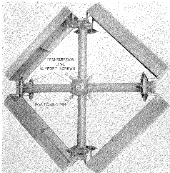
Fig. 3—Bottom view of loop.
