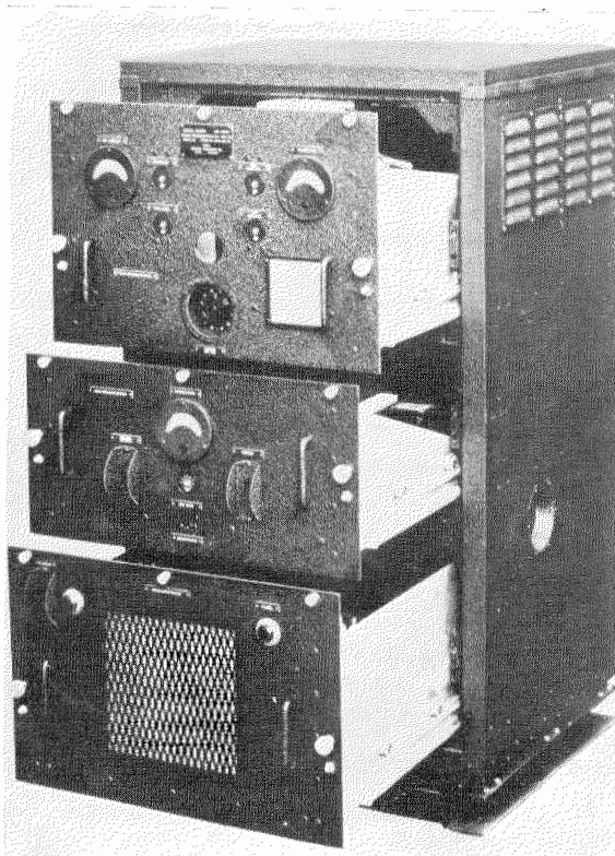
Fig. 12—The radio-frequency, power-supply, and modulator sections of the localizer transmitter are mounted in the three "drawers" shown above.
