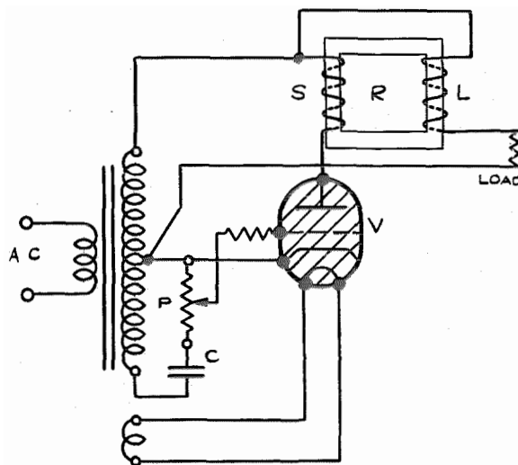
Fig. 44—Reactor control of alternating-current load.
