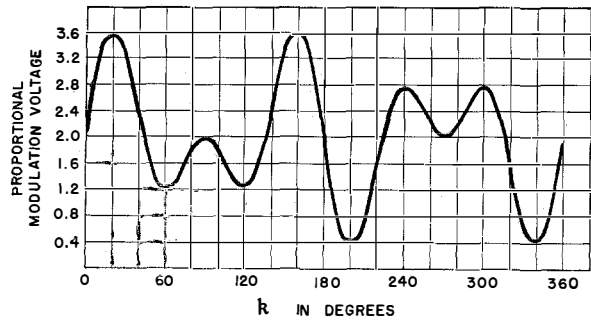
Fig. 42—Phase relations of radiated signals from upper and lower antennas.
