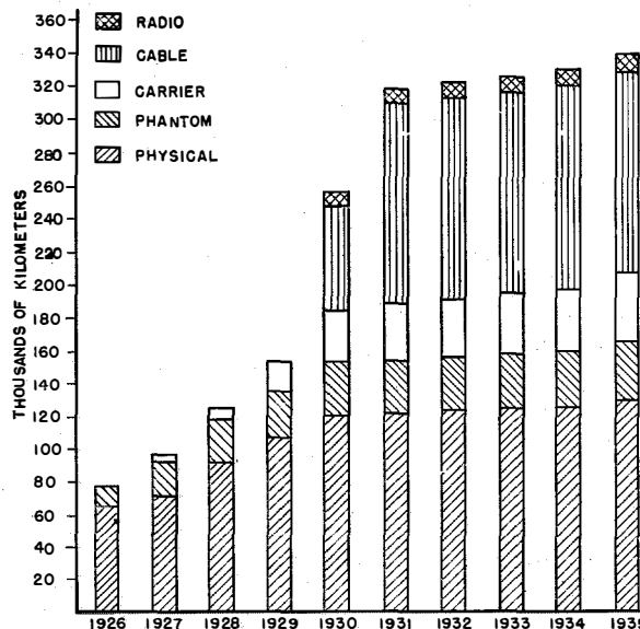
Fig. 7—Total length of toll circuits from 1926 through 1935, when the Civil War started. Unsettled conditions have prevented substantial expansion since then.
