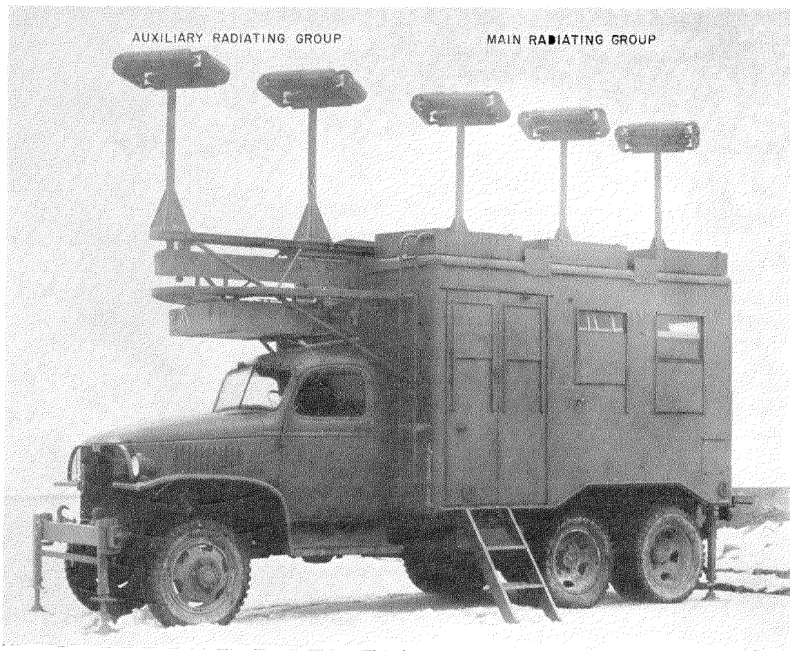
Fig. 7—Localizer truck with loops in operating position.
