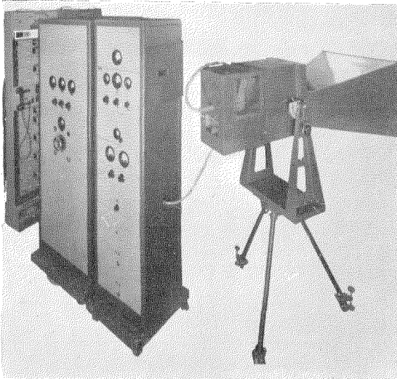
Fig. 15—Multi-channel transmitter.
