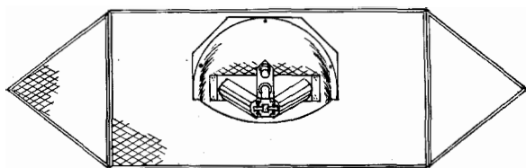
Fig. 25—Screen and lower antenna of glide-path equipment.
