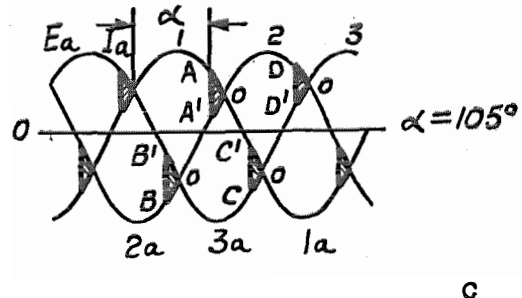
Fig. 46—Voltage conditions in 3-phase full-wave series-circuit rectifier, with resistive load.
