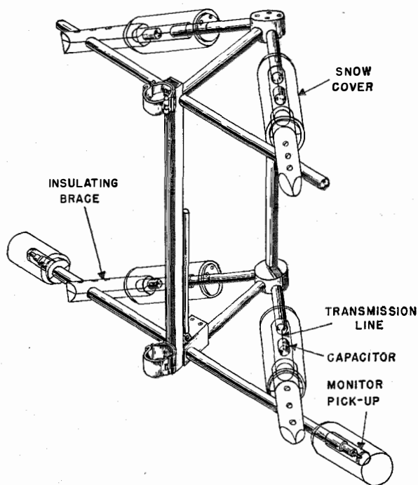
Fig. 26—Upper antenna of the glide-path equipment.
