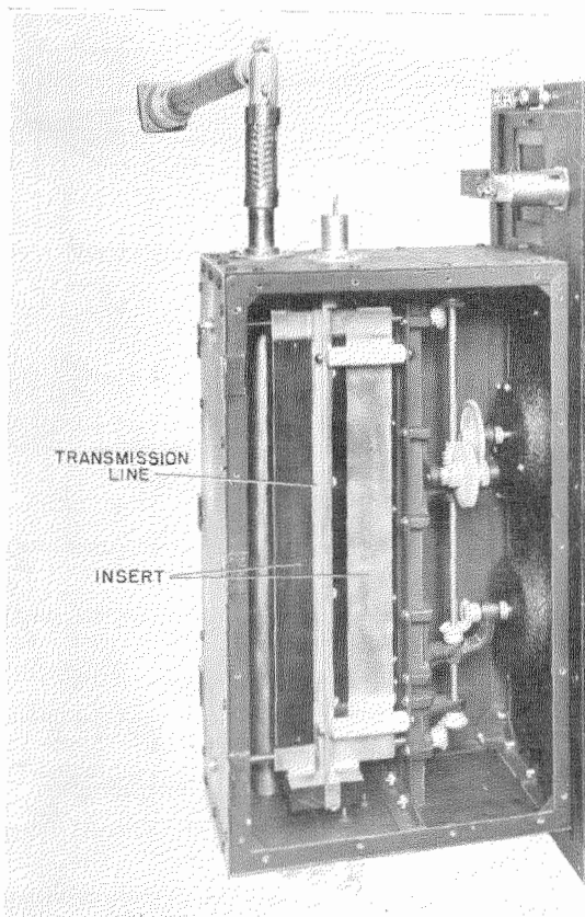
Fig. 41—Phasing unit with cover removed.
