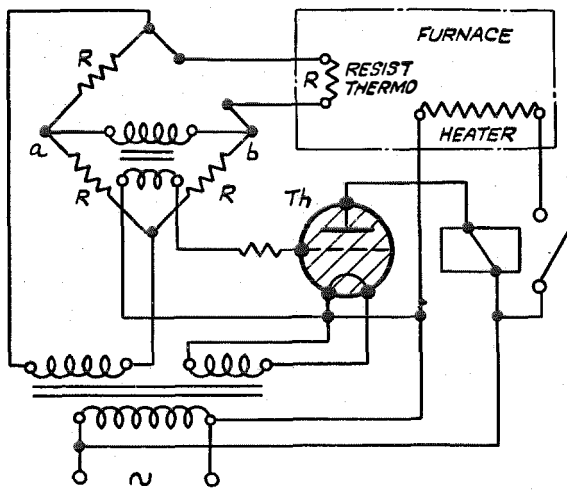
Fig. 12—High-temperature control.
