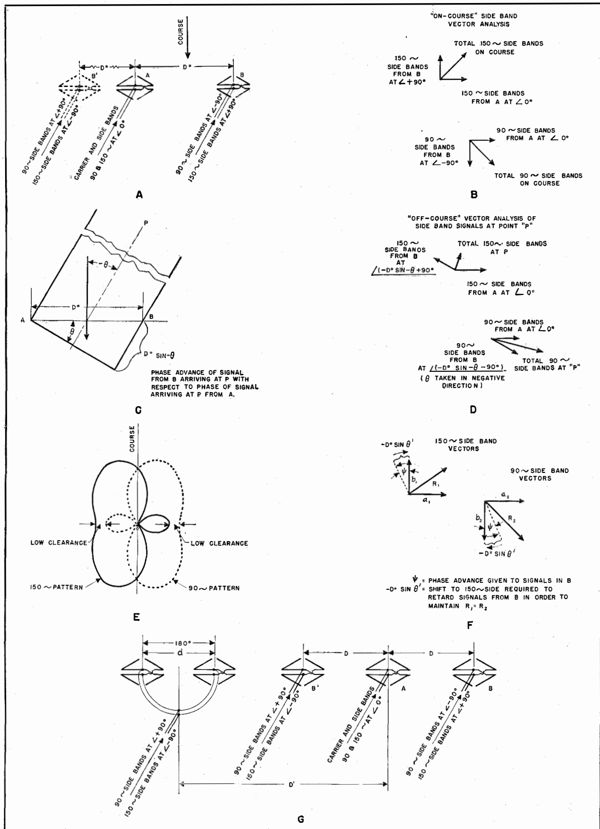
Fig. 37—Vector analyses of side bands for "on-course" and "off-course" conditions.
