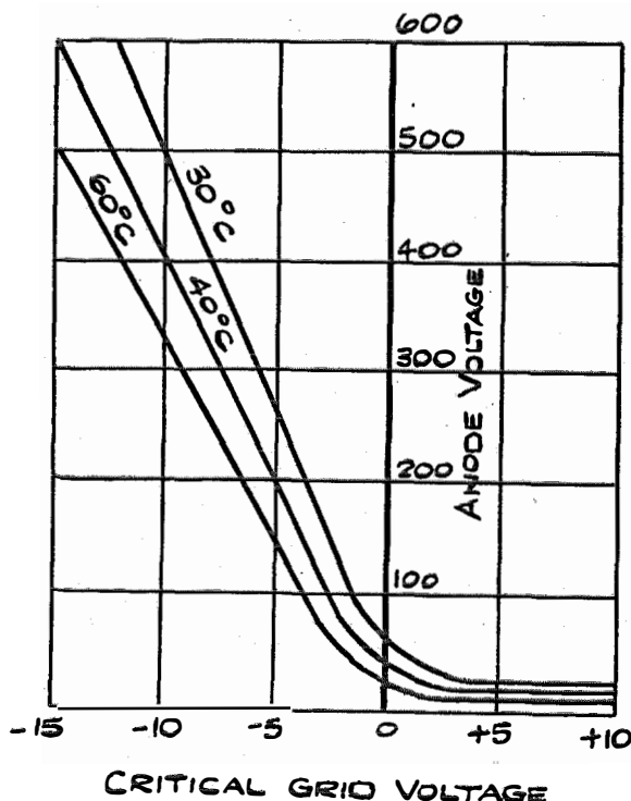
Fig. 3—Grid-voltage—anode-voltage characteristic of a typical thyratron. The critical grid voltage is that at which ionisation occurs.
