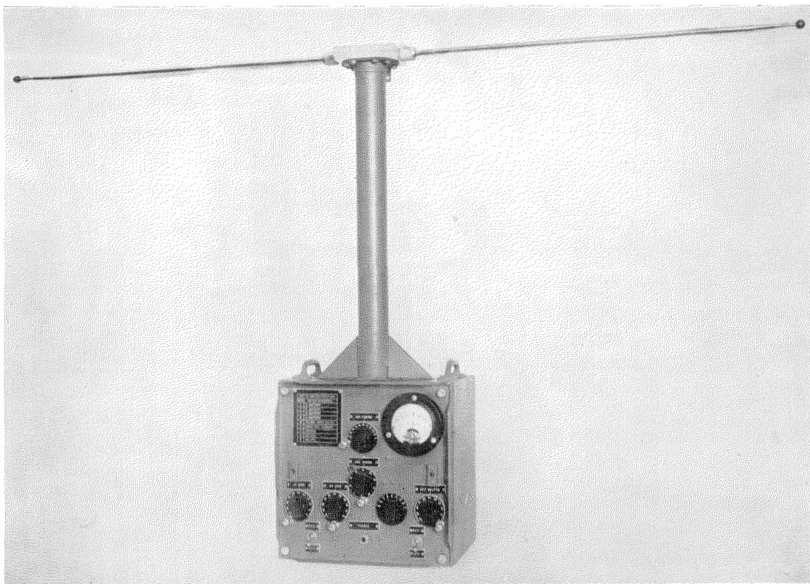
Fig. 14—The portable course detector is the most useful piece of test equipment in adjusting the localizer.
