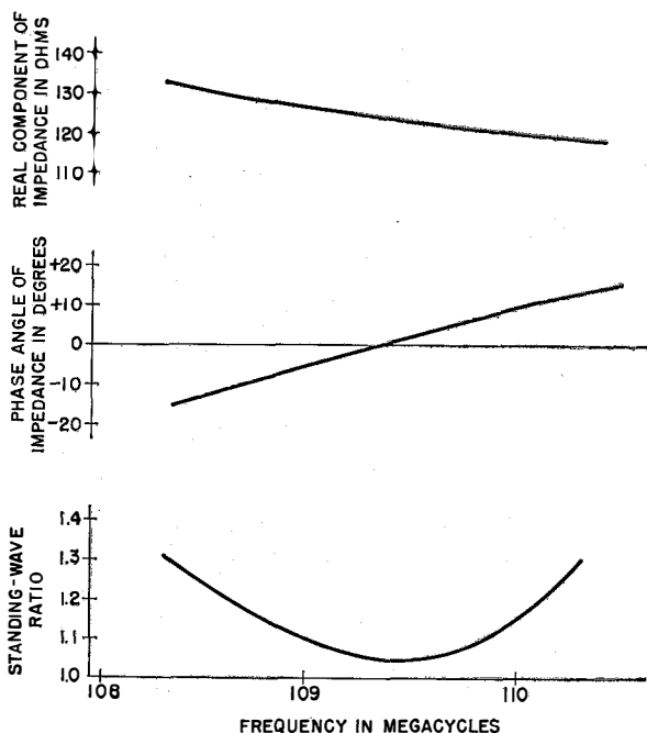
Fig. 4—Real component and phase angle of impedance and standing-wave ratio plotted against frequency for the broad-band loop.
